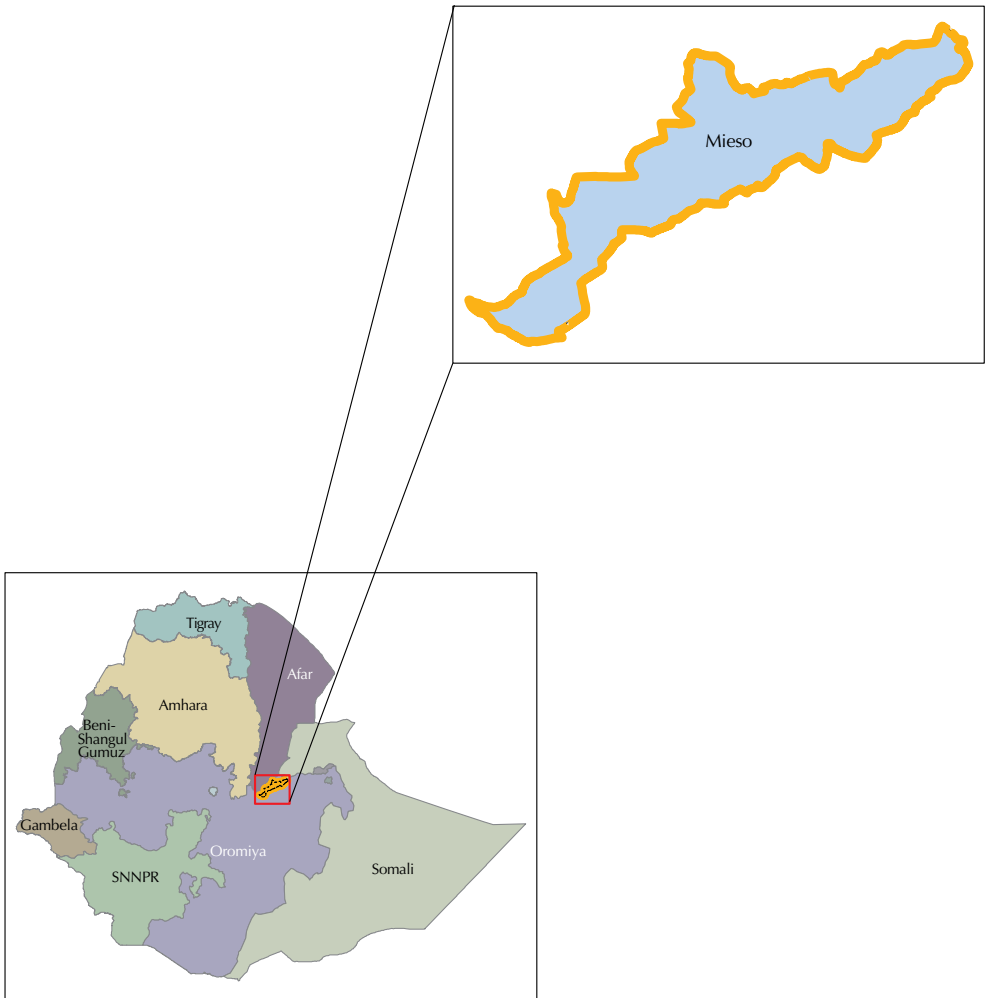
Figure 1. Elevation map of Mieso district, Oromia Region, Ethiopia.
